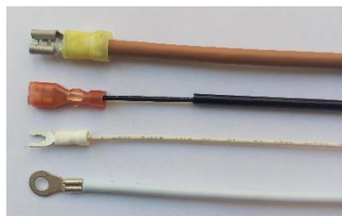
terminal wire harness
