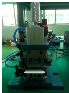
Large wire pneumatic stripping machines
